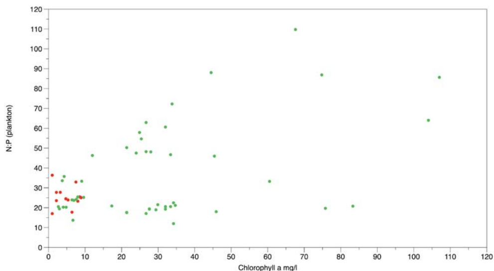
Figure 3.10. N/P ratio of particulate nitrogen and phosphorus (calculated as TN or TP minus dissolved nitrogen or phosphorus) as a function of planktonic chlorophyll a . Green dots are Lady's Island Lake; red dots are the control site. At low planktonic chlorophyll a , N/P approaches the Redfield ratio of 16:1.
