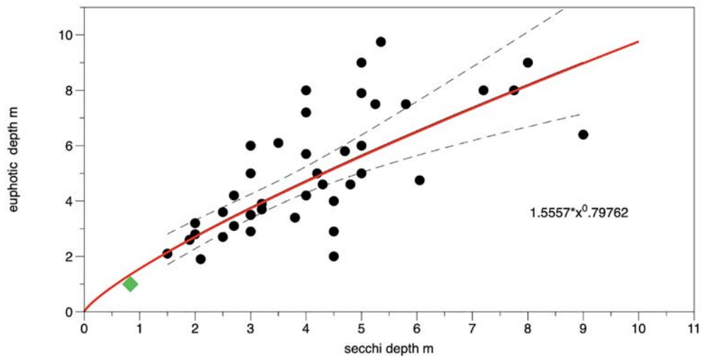
Figure 3.4. The relationship between Secchi depth and euphotic depth (maximum depth of vegetation) based on recent Irish lake surveys (Roden et al. , 2020, 2021). The average value derived from the CLEAR project for Lady's Island Lake is shown for comparison (green diamond).
